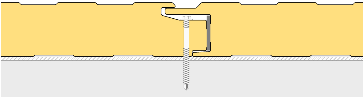
ISOPARETE PLUS PG joint (approximately 22 mm leak)
