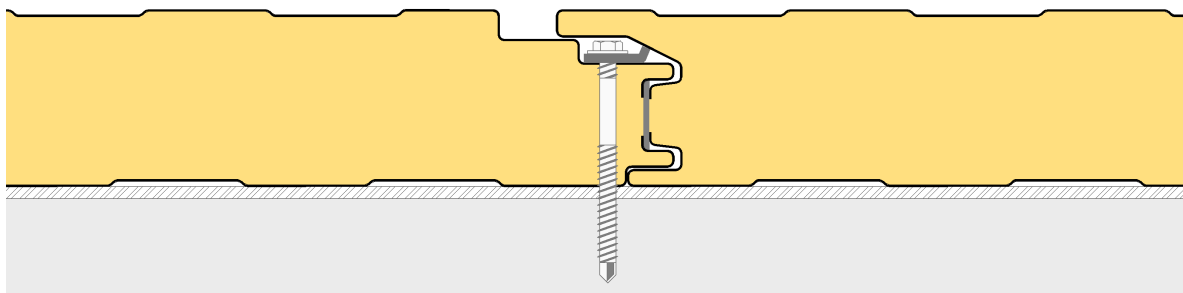
ISOPARETE PLUS PG joint (approximately 22 mm leak)
